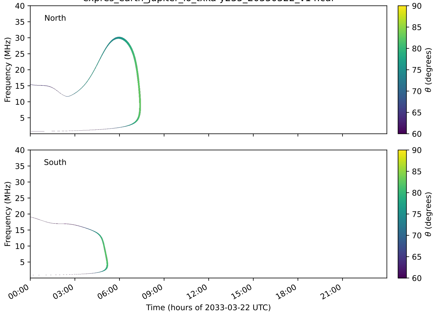
expres_earth_jupiter_io_txka-y235_20330322_v14.cdf
