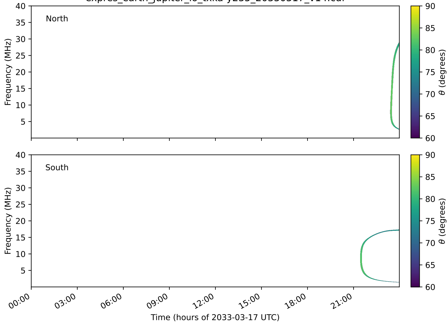
expres_earth_jupiter_io_txka-y235_20330317_v14.cdf
