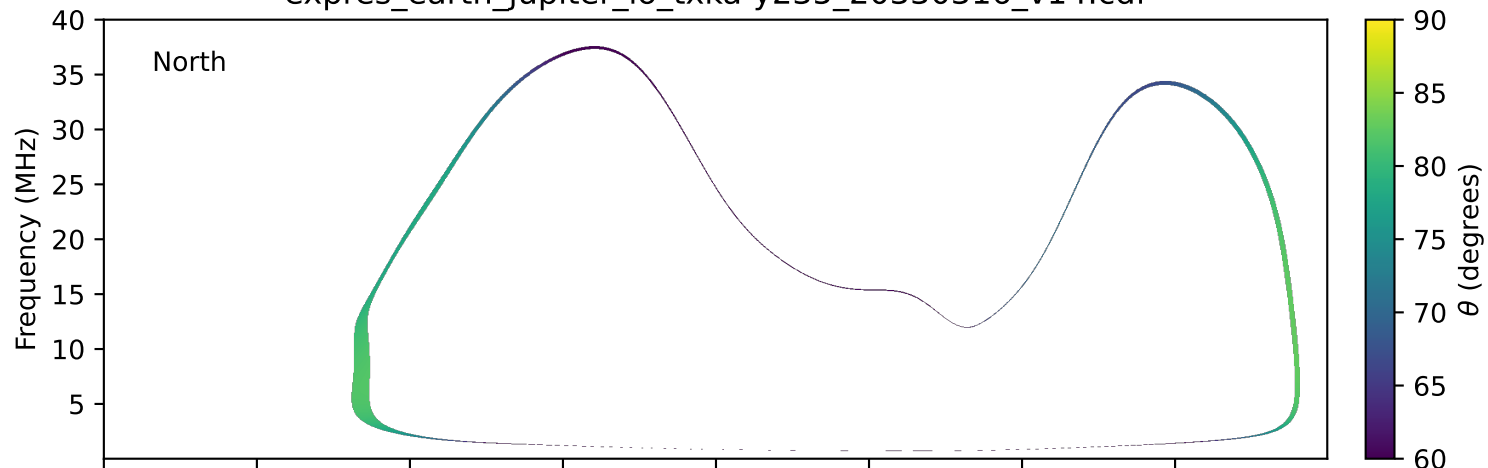
expres_earth_jupiter_io_txka-y235_20330316_v14.cdf
