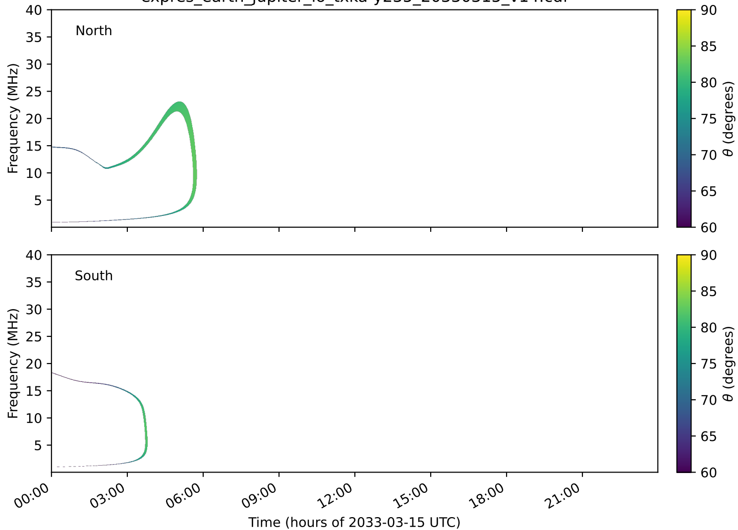
expres_earth_jupiter_io_txka-y235_20330315_v14.cdf
