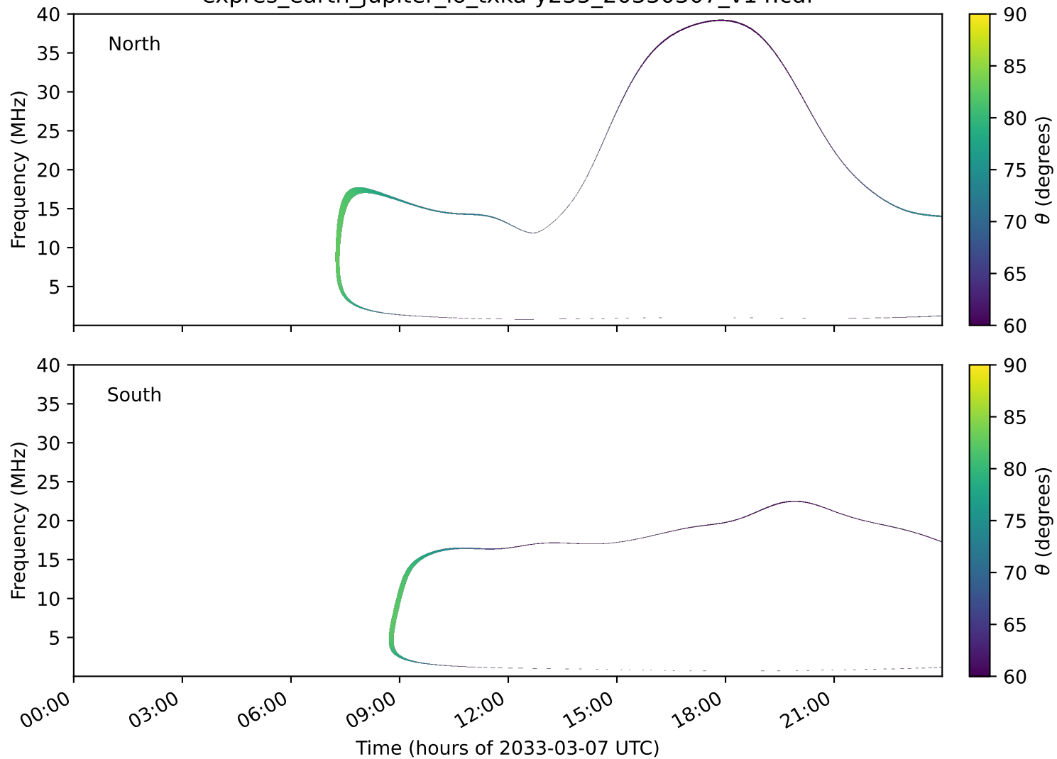
expres_earth_jupiter_io_txka-y235_20330307_v14.cdf
