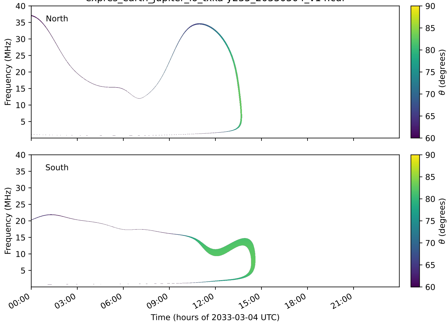
expres_earth_jupiter_io_txka-y235_20330304_v14.cdf
