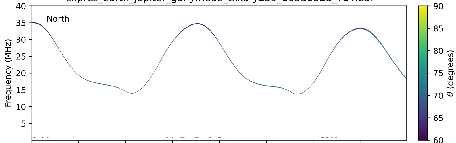
expres_earth_jupiter_ganymede_txka-y235_20330328_v14.cdf
