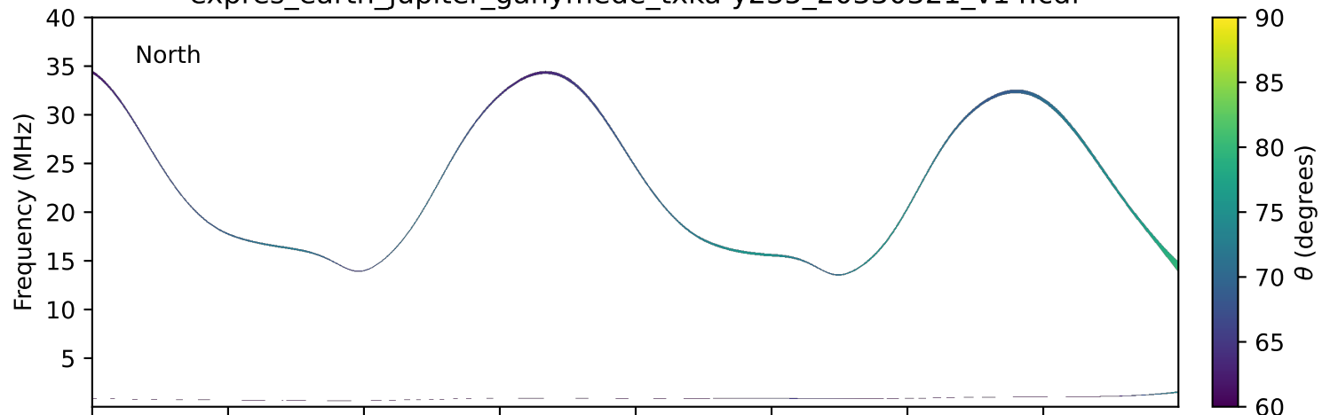
expres_earth_jupiter_ganymede_txka-y235_20330321_v14.cdf
