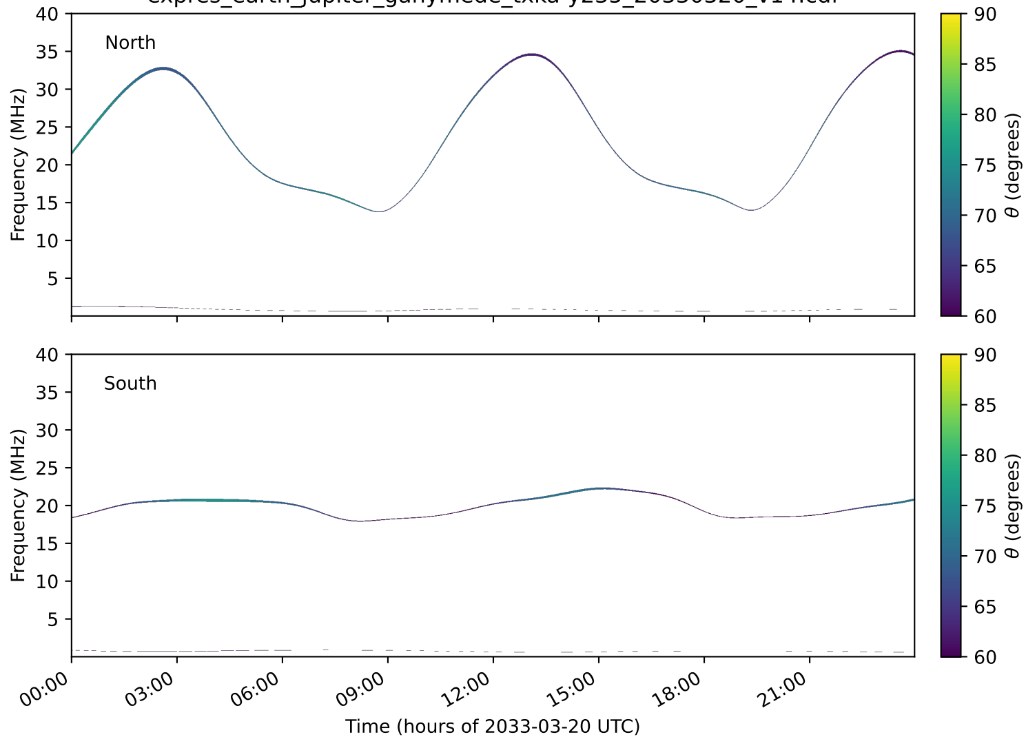
expres_earth_jupiter_ganymede_txka-y235_20330320_v14.cdf
