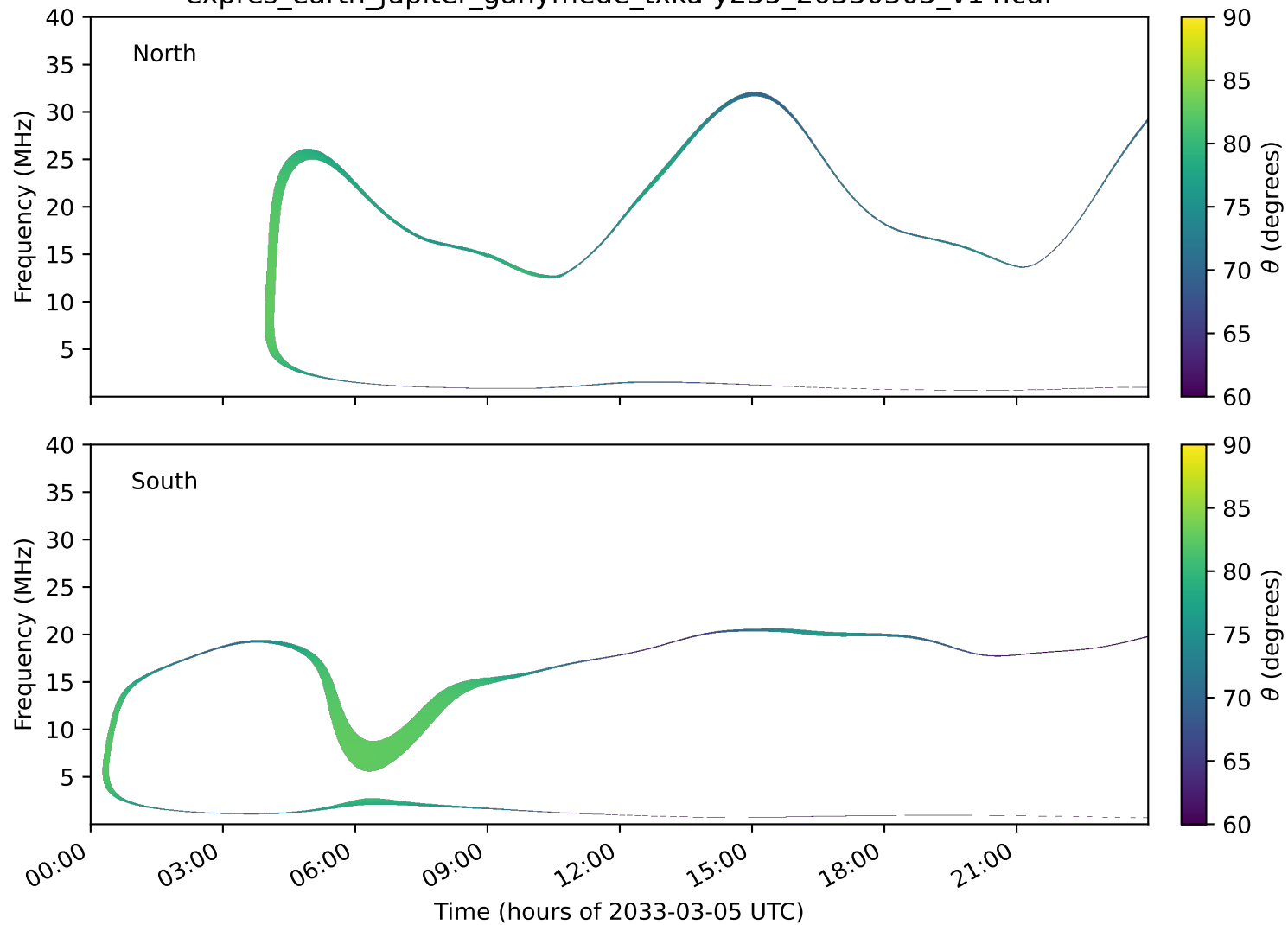
expres_earth_jupiter_ganymede_txka-y235_20330305_v14.cdf
