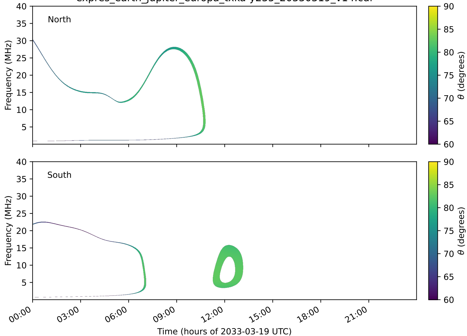
expres_earth_jupiter_europa_txka-y235_20330319_v14.cdf
