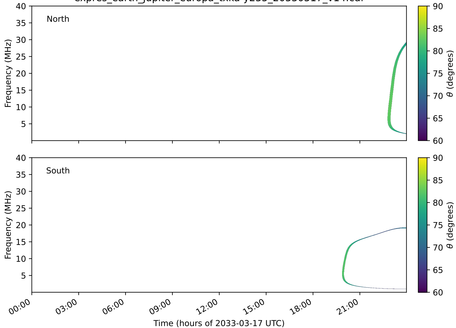
expres_earth_jupiter_europa_txka-y235_20330317_v14.cdf
