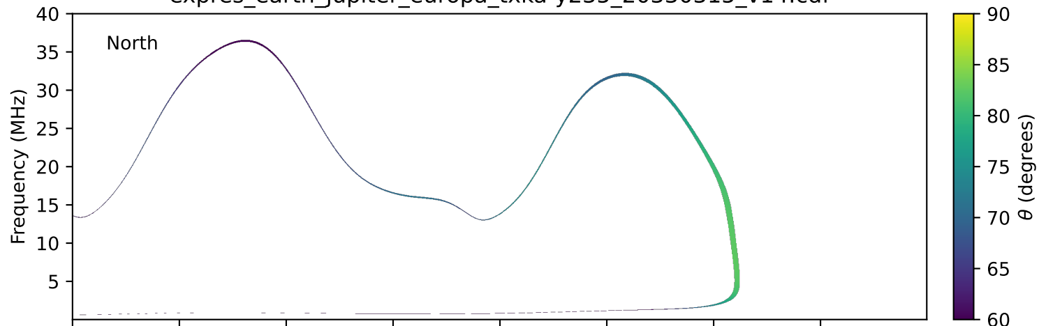
expres_earth_jupiter_europa_txka-y235_20330315_v14.cdf
