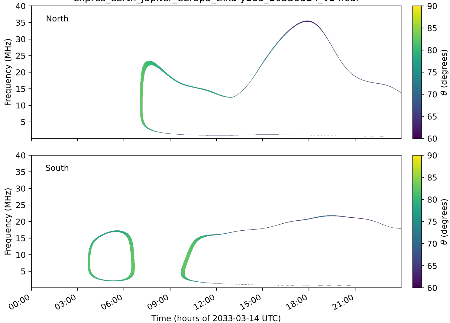
expres_earth_jupiter_europa_txka-y235_20330314_v14.cdf
