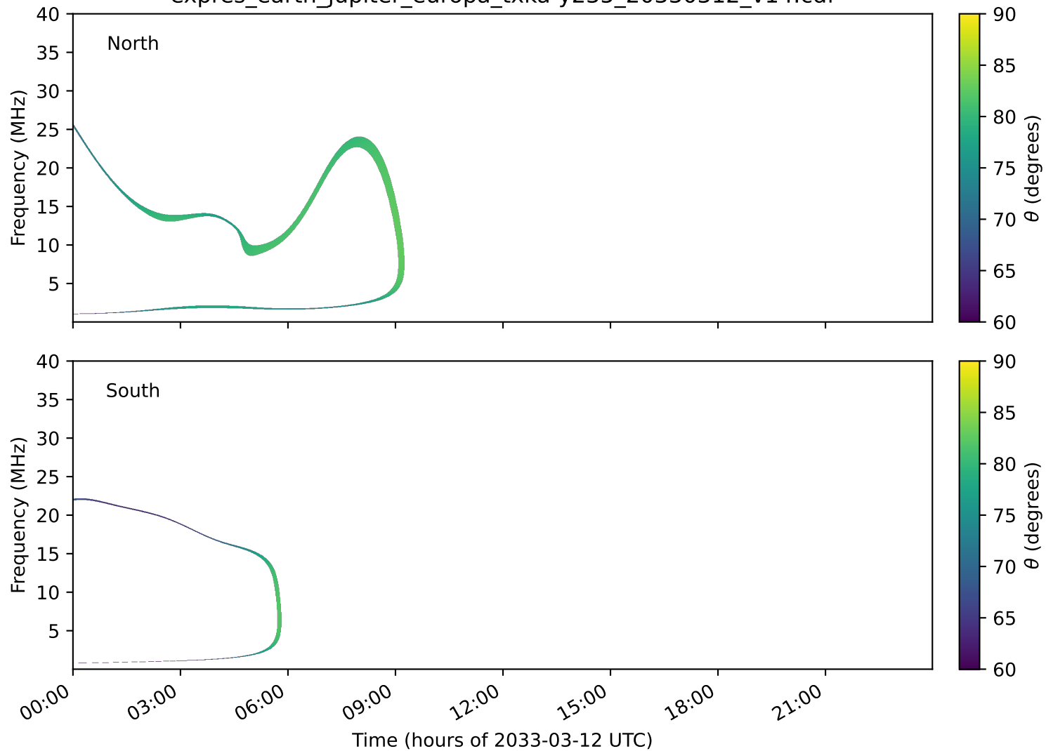
expres_earth_jupiter_europa_txka-y235_20330312_v14.cdf
