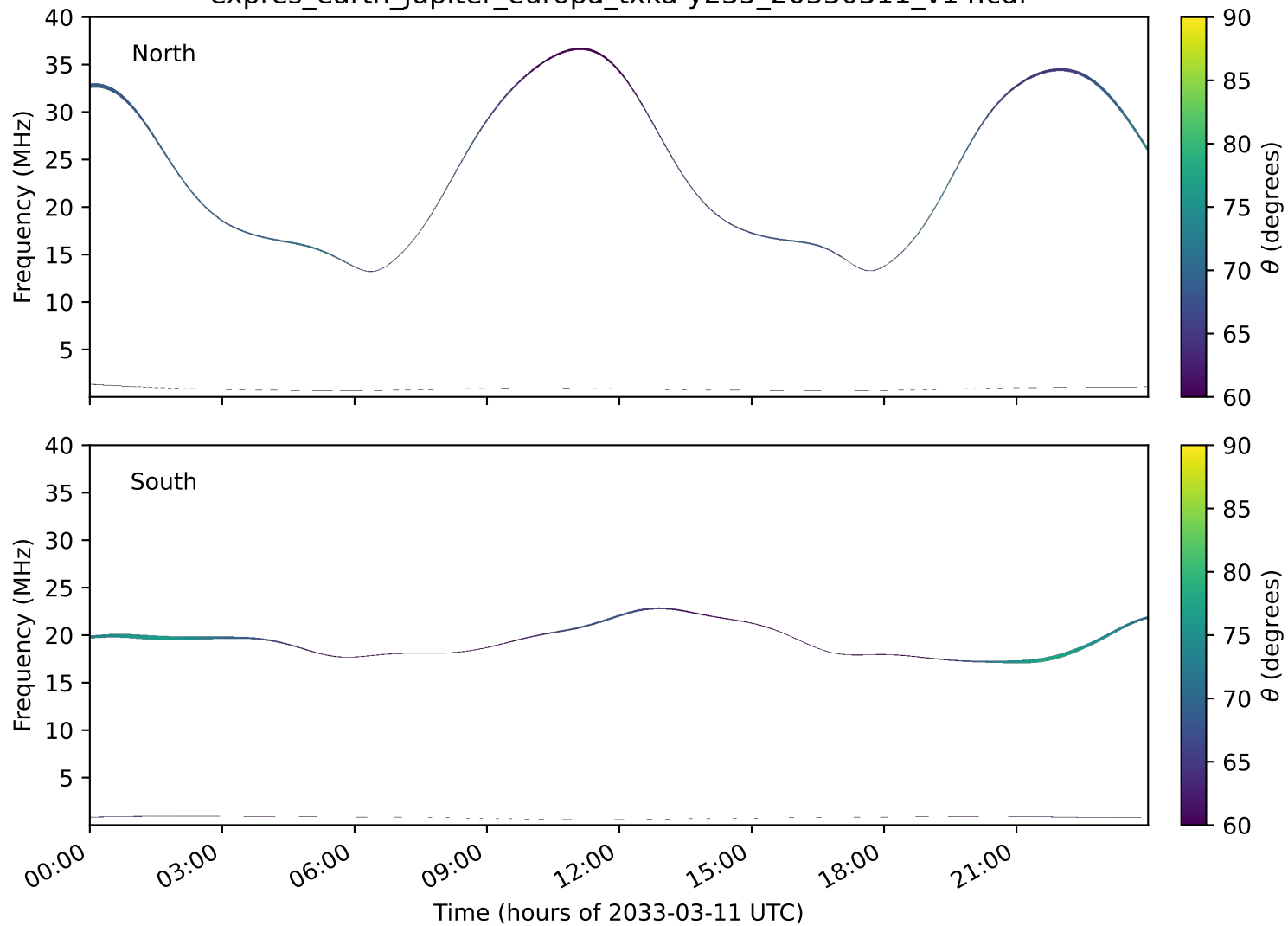
expres_earth_jupiter_europa_txka-y235_20330311_v14.cdf
