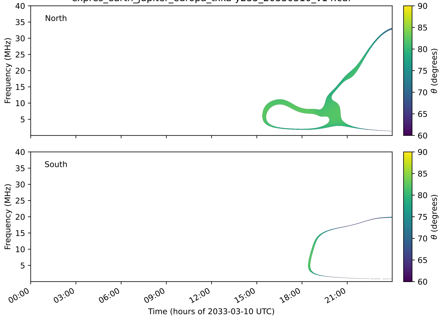
expres_earth_jupiter_europa_txka-y235_20330310_v14.cdf
