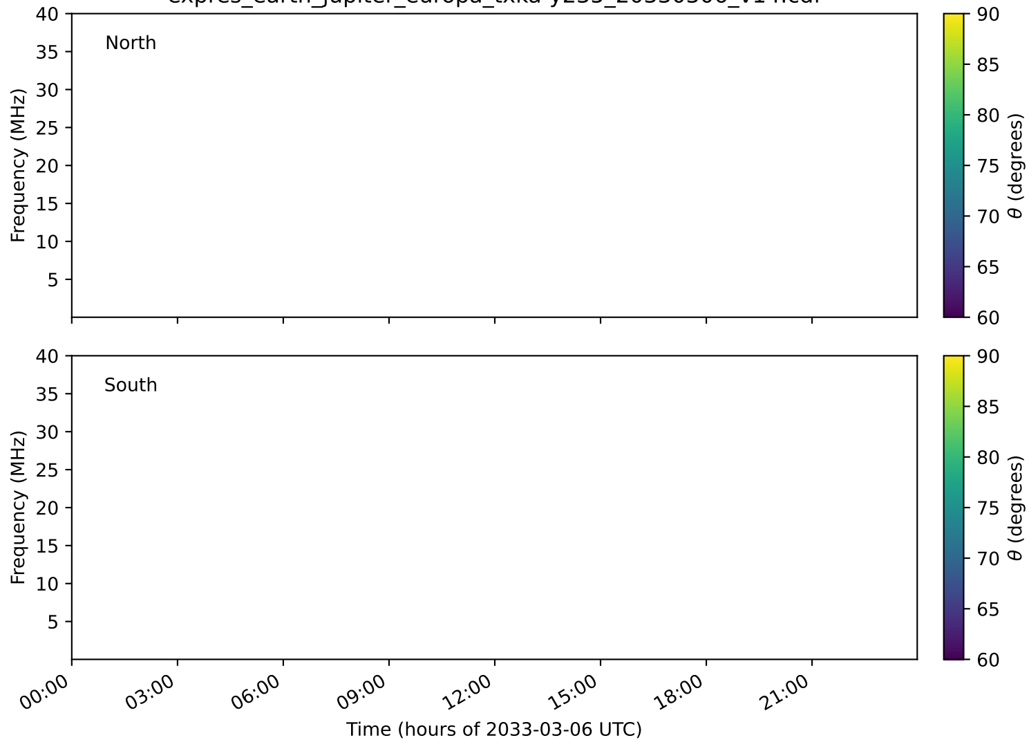
expres_earth_jupiter_europa_txka-y235_20330306_v14.cdf
