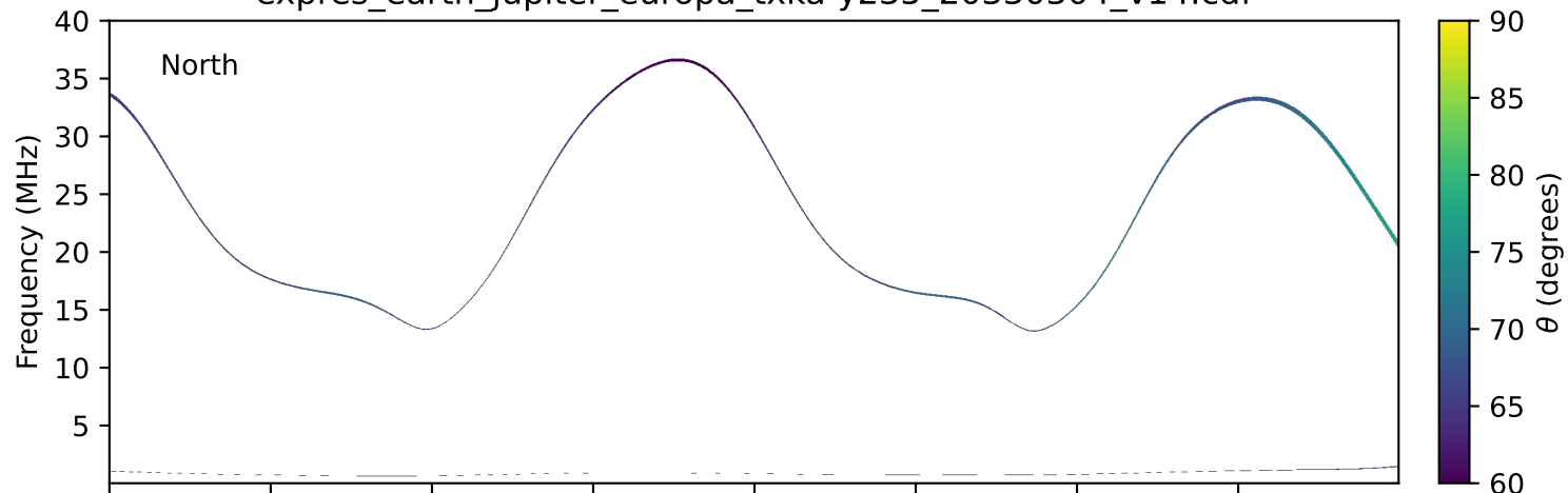
expres_earth_jupiter_europa_txka-y235_20330304_v14.cdf
