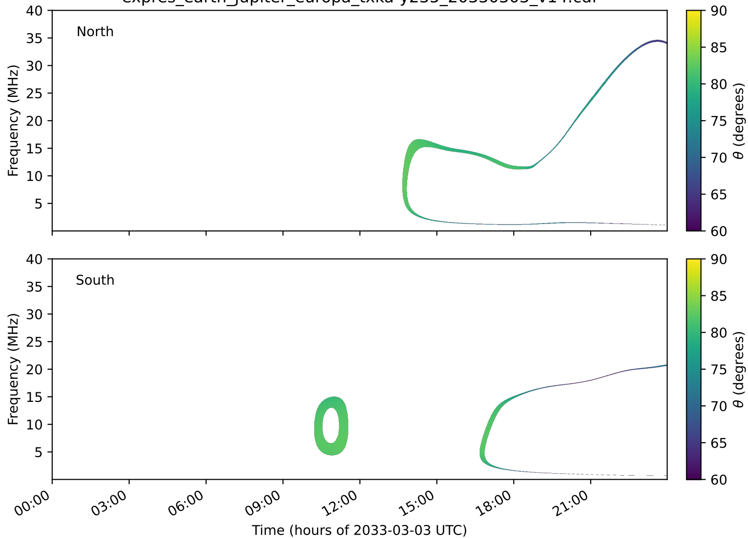
expres_earth_jupiter_europa_txka-y235_20330303_v14.cdf
