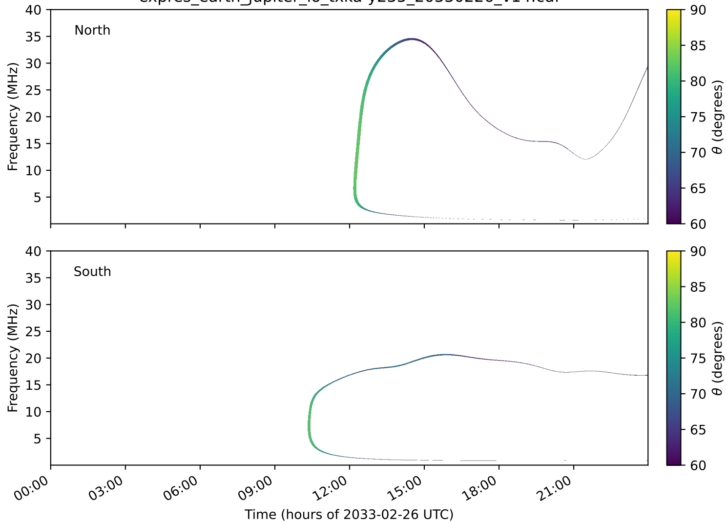
expres_earth_jupiter_io_txka-y235_20330226_v14.cdf
