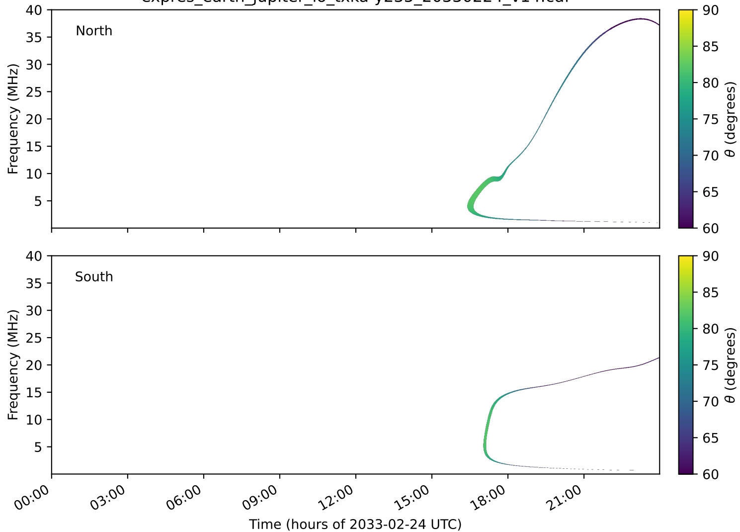
expres_earth_jupiter_io_txka-y235_20330224_v14.cdf
