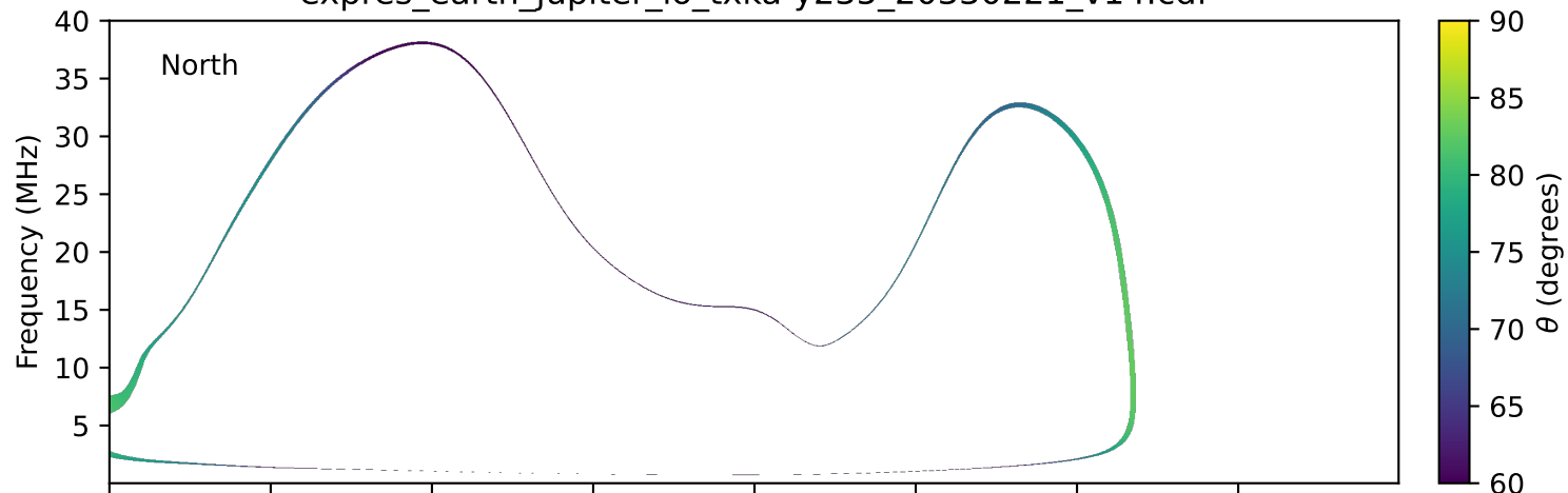
expres_earth_jupiter_io_txka-y235_20330221_v14.cdf
