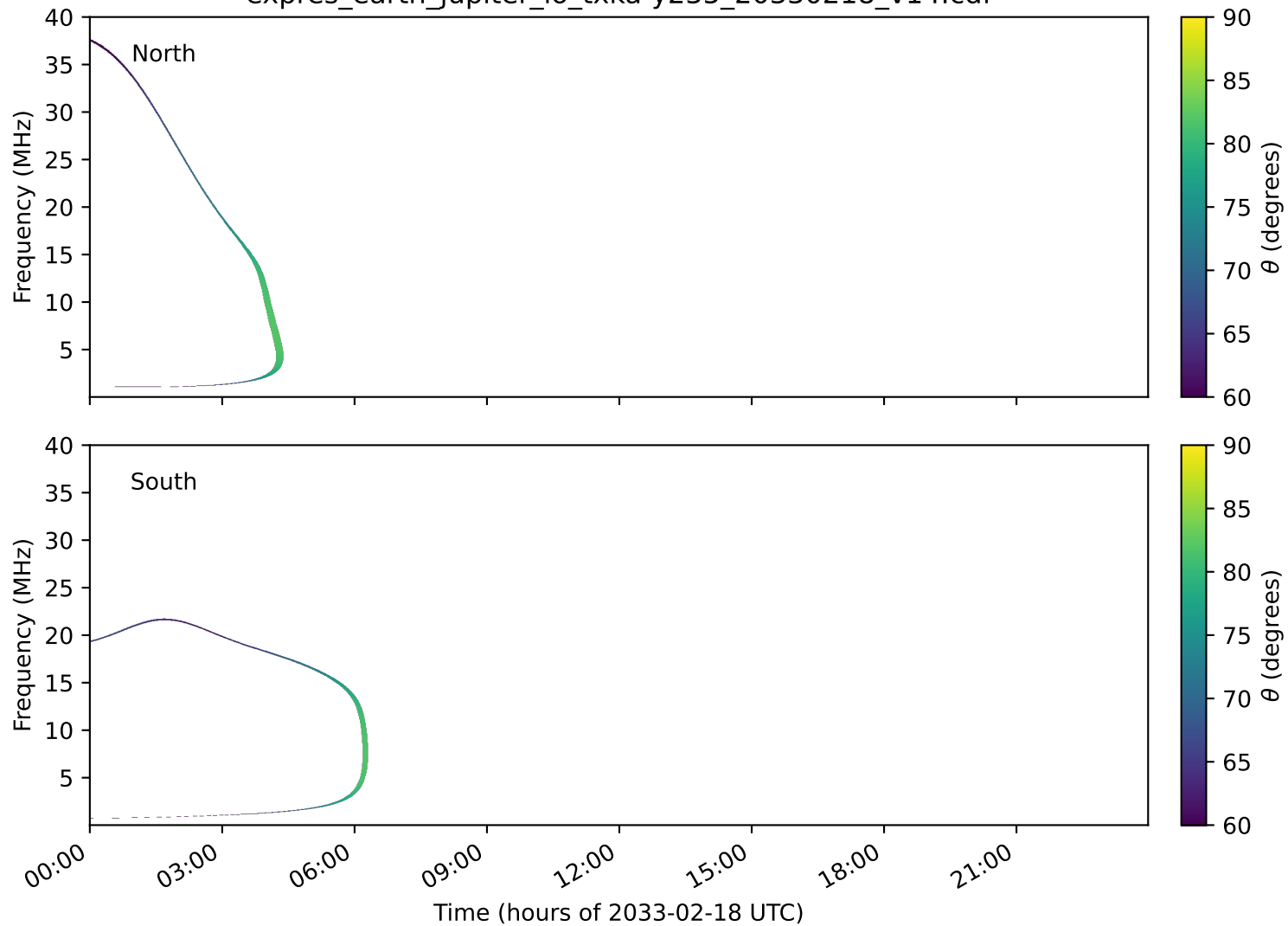
expres_earth_jupiter_io_txka-y235_20330218_v14.cdf
