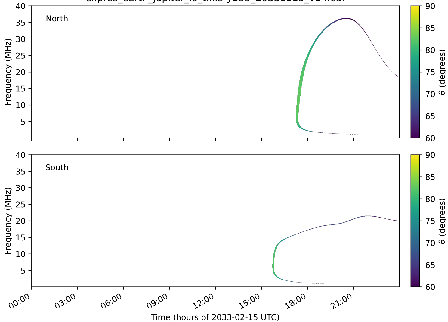
expres_earth_jupiter_io_txka-y235_20330215_v14.cdf
