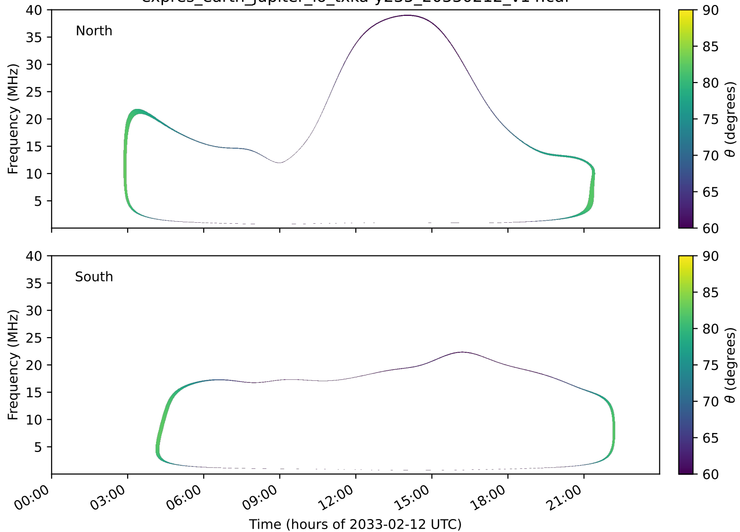
expres_earth_jupiter_io_txka-y235_20330212_v14.cdf
