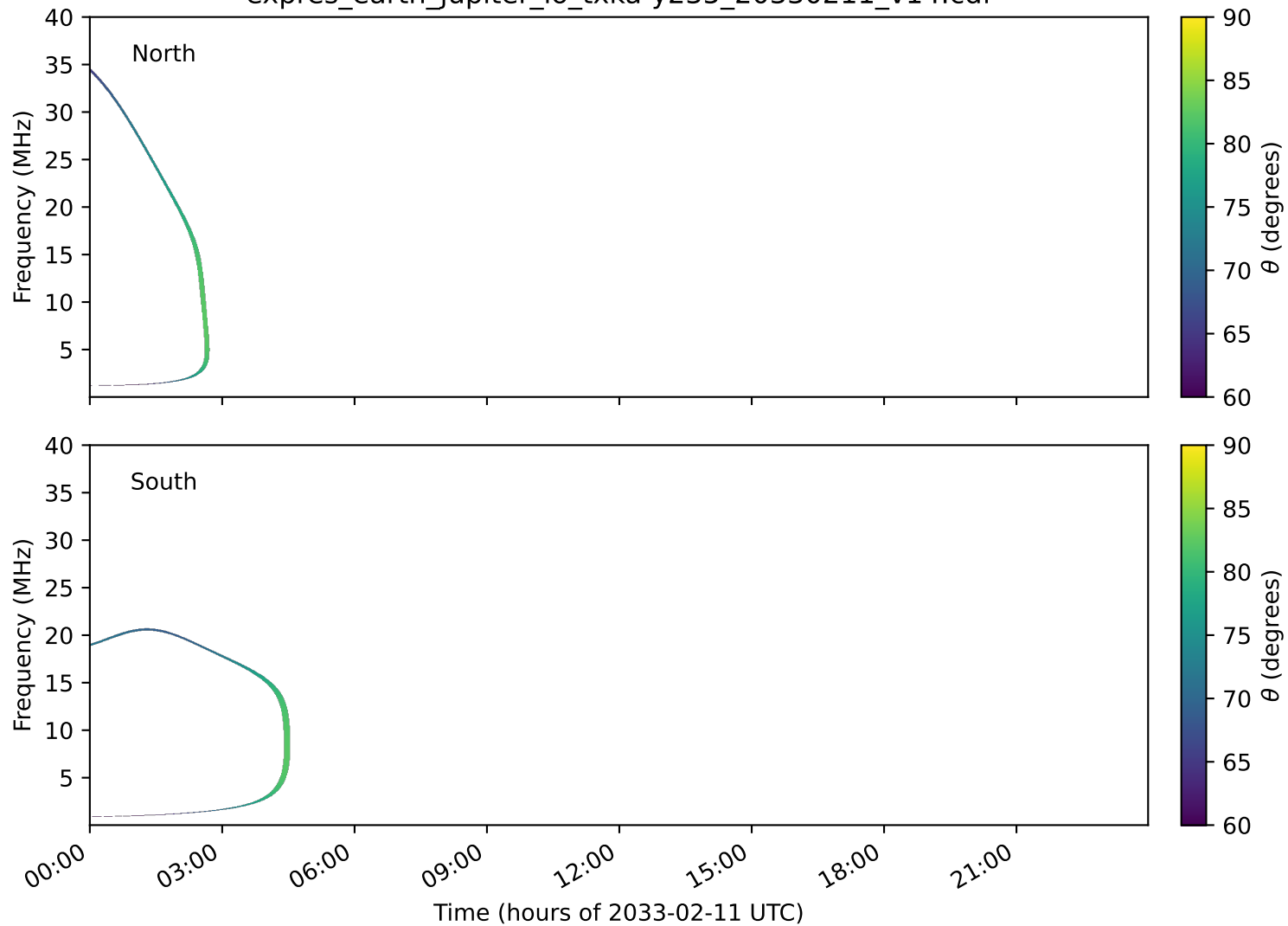
expres_earth_jupiter_io_txka-y235_20330211_v14.cdf
