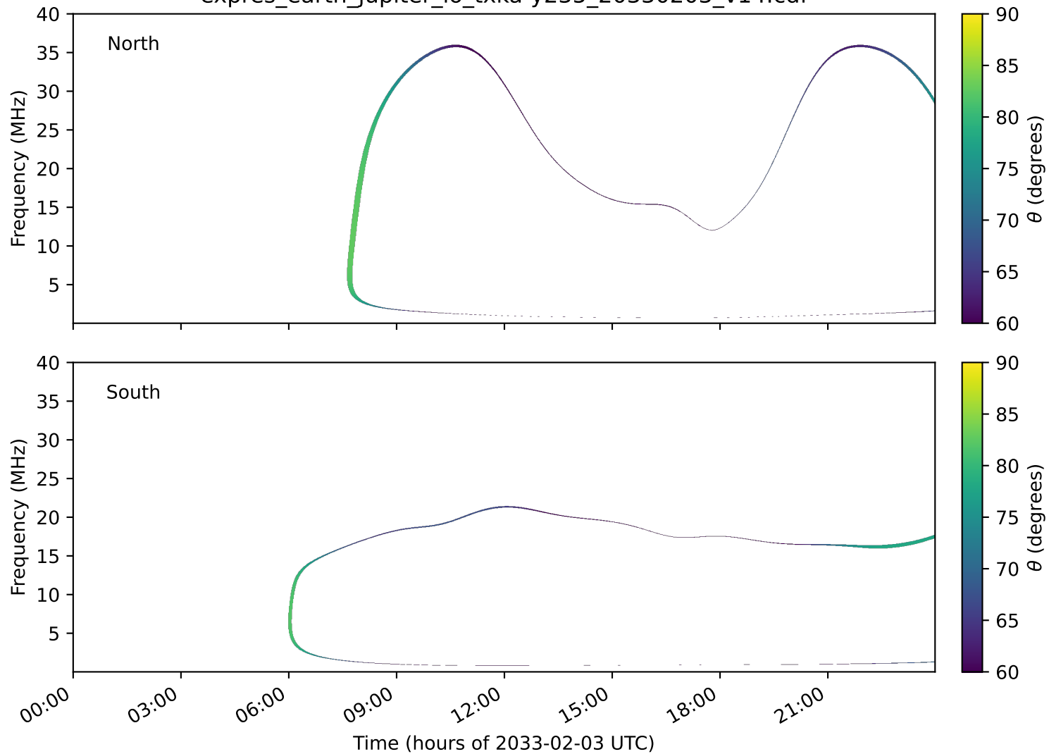
expres_earth_jupiter_io_txka-y235_20330203_v14.cdf
