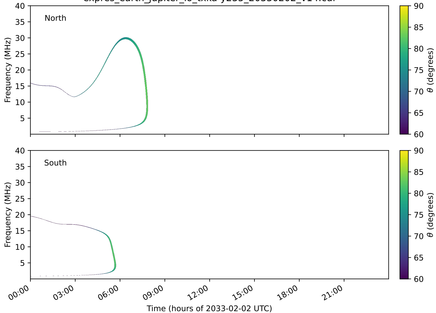
expres_earth_jupiter_io_txka-y235_20330202_v14.cdf
