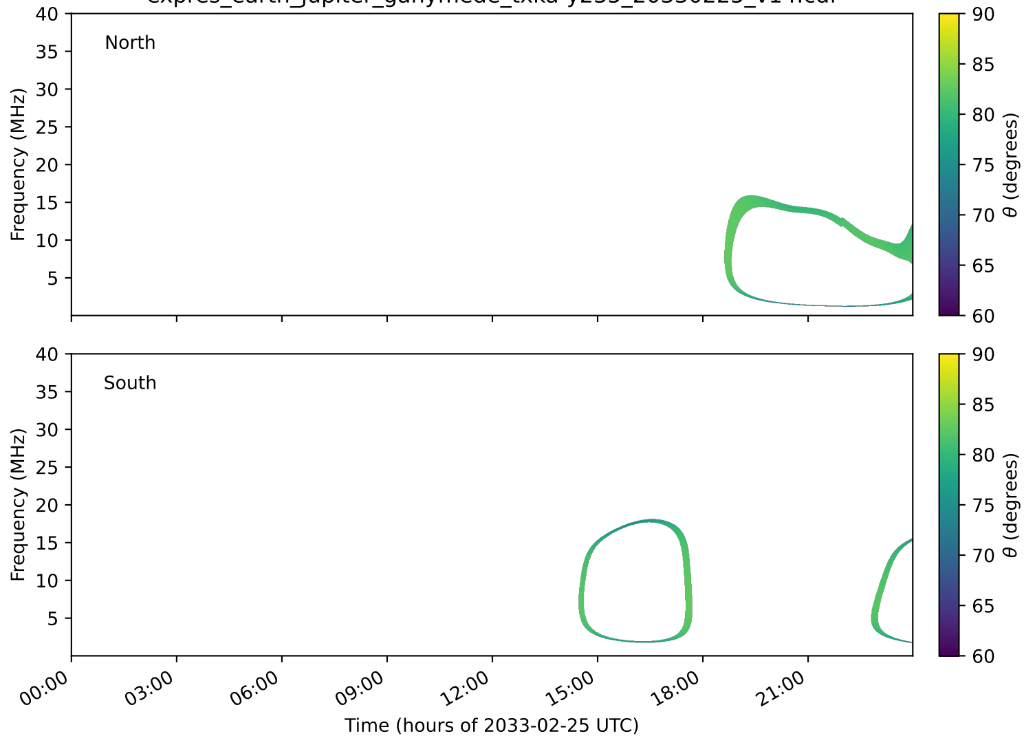
expres_earth_jupiter_ganymede_txka-y235_20330225_v14.cdf
