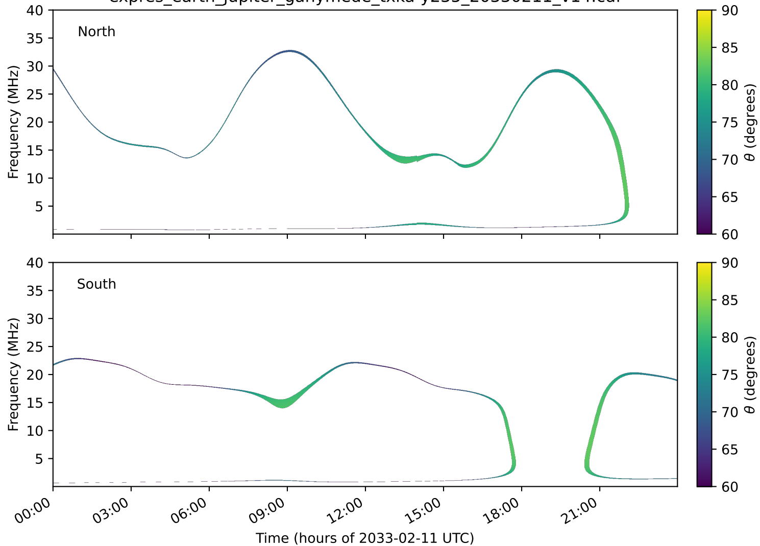
expres_earth_jupiter_ganymede_txka-y235_20330211_v14.cdf
