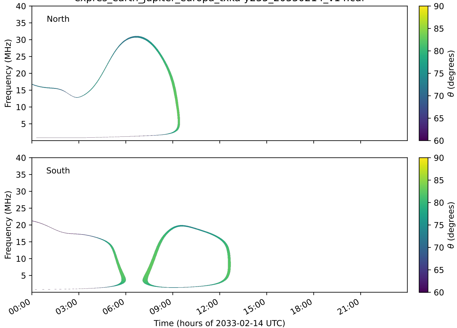
expres_earth_jupiter_europa_txka-y235_20330214_v14.cdf
