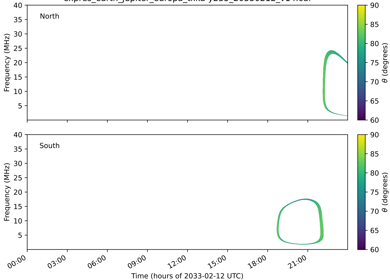
expres_earth_jupiter_europa_txka-y235_20330212_v14.cdf
