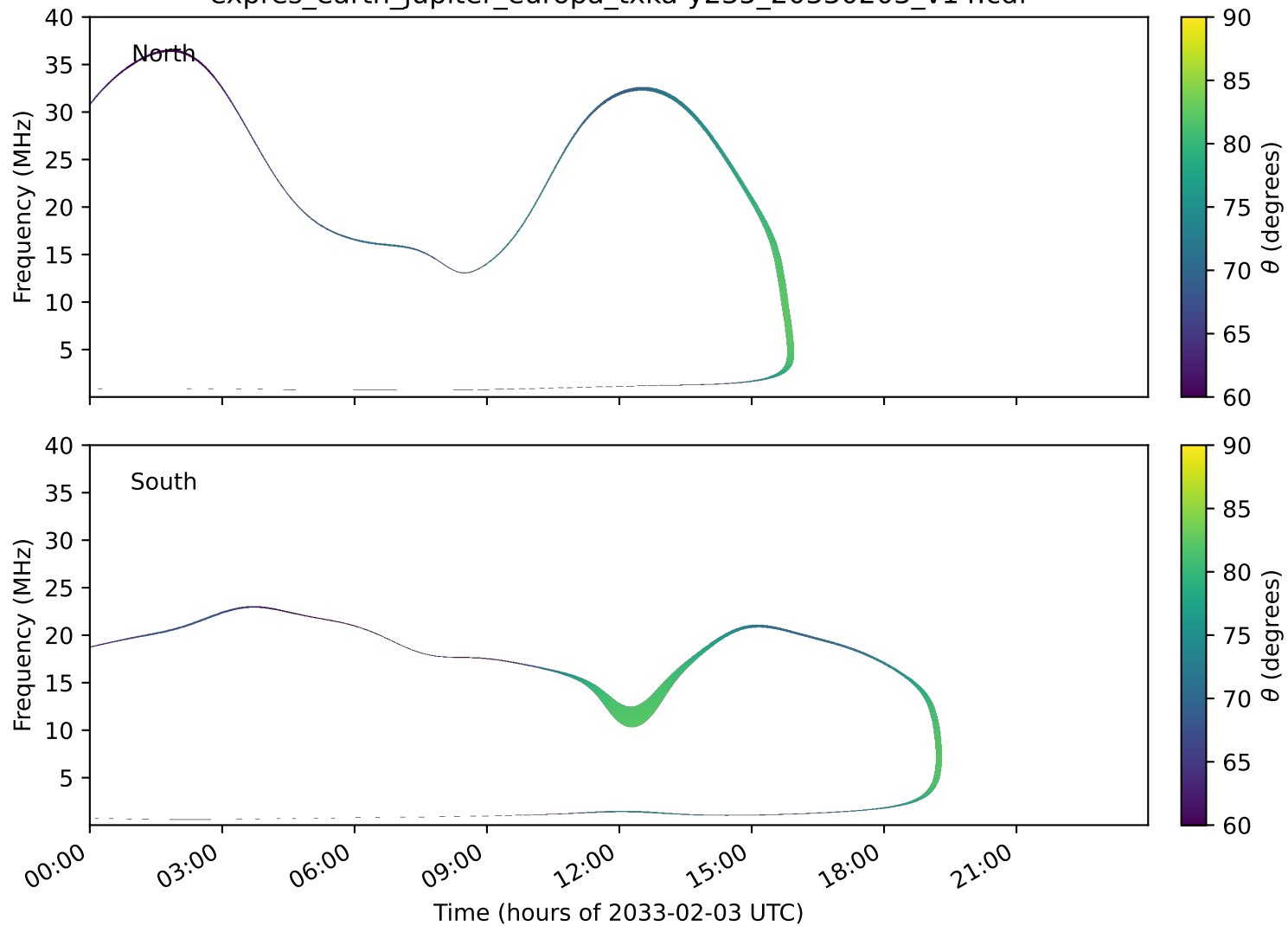
expres_earth_jupiter_europa_txka-y235_20330203_v14.cdf
