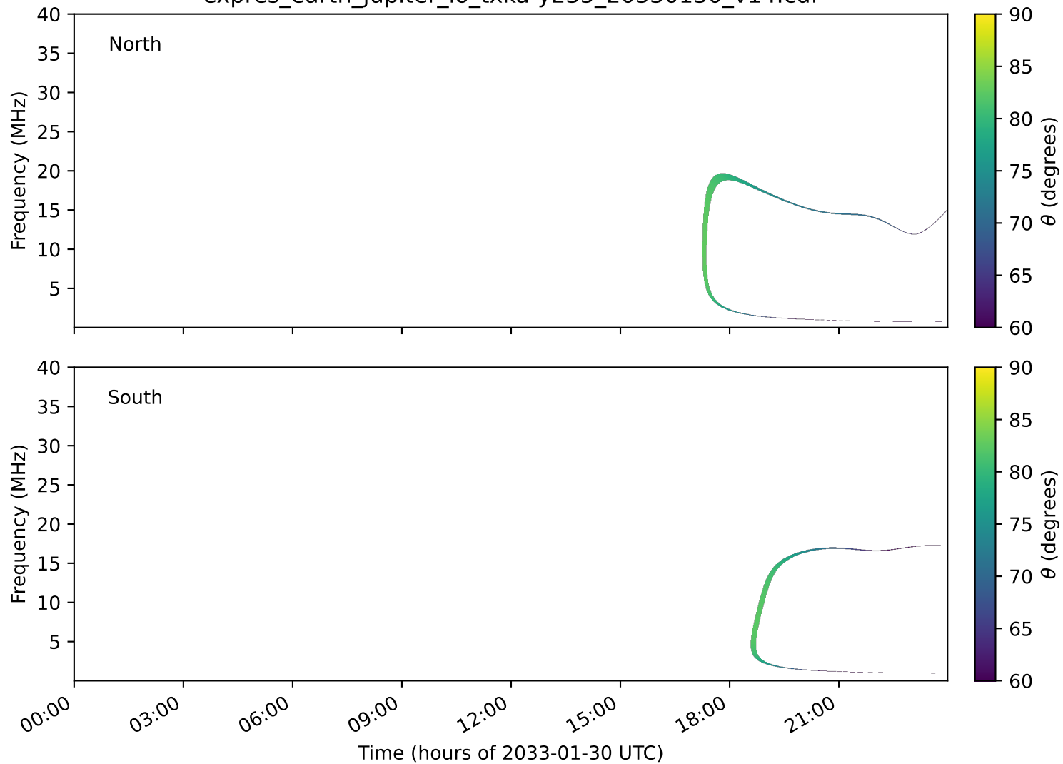
expres_earth_jupiter_io_txka-y235_20330130_v14.cdf
