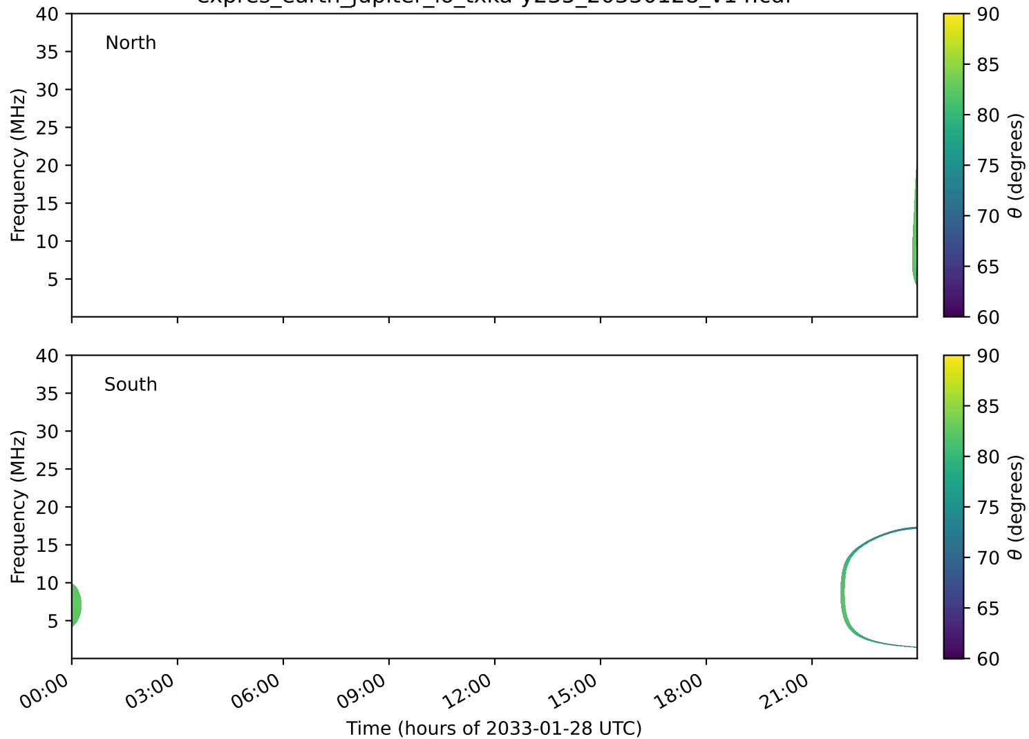
expres_earth_jupiter_io_txka-y235_20330128_v14.cdf
