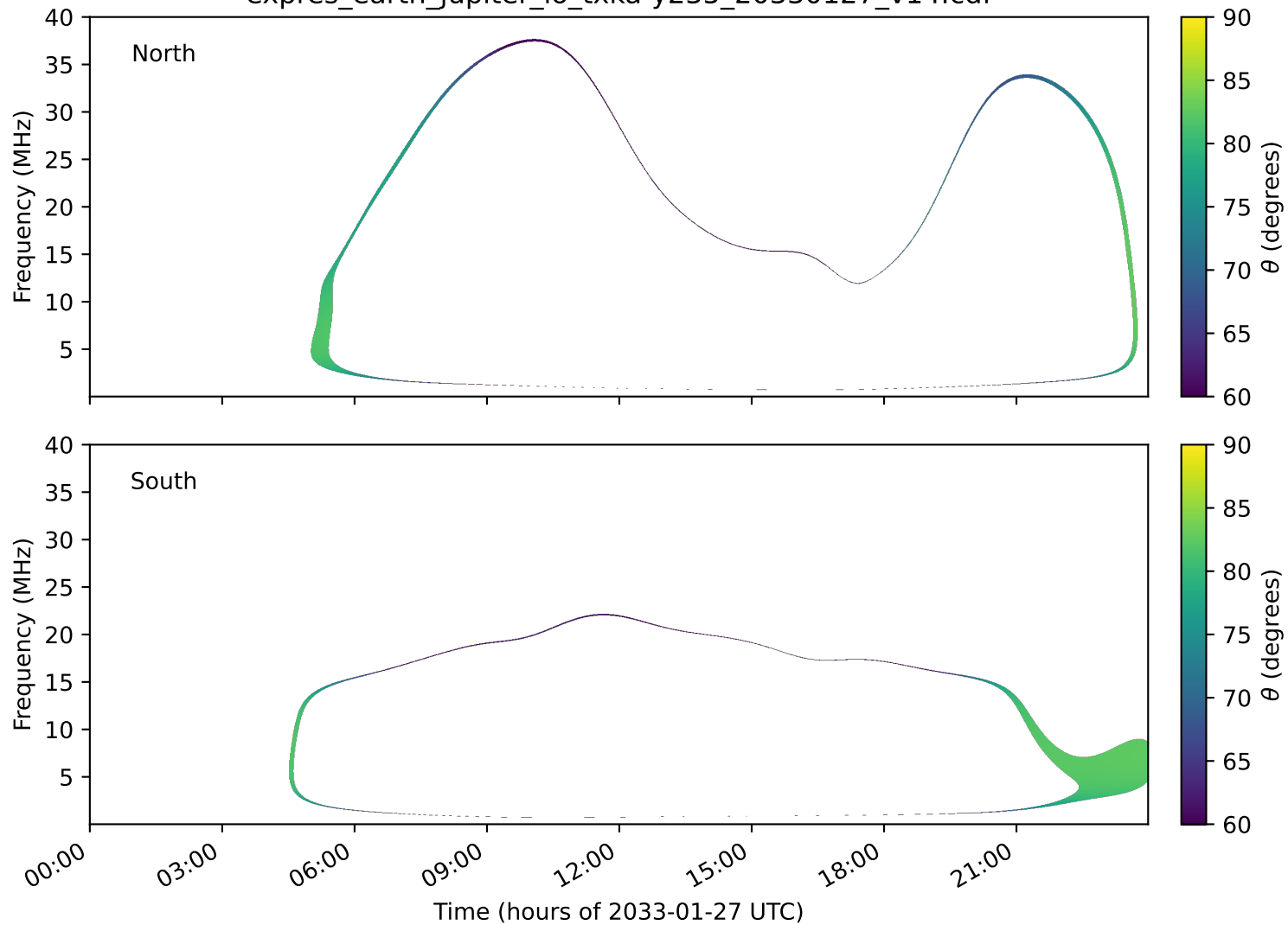
expres_earth_jupiter_io_txka-y235_20330127_v14.cdf
