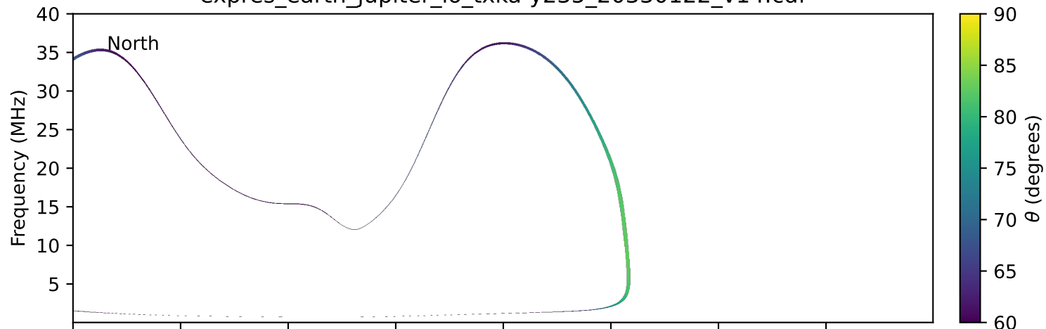
expres_earth_jupiter_io_txka-y235_20330122_v14.cdf
