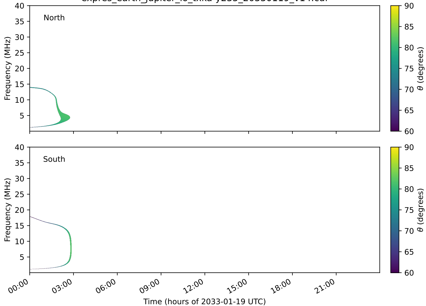
expres_earth_jupiter_io_txka-y235_20330119_v14.cdf
