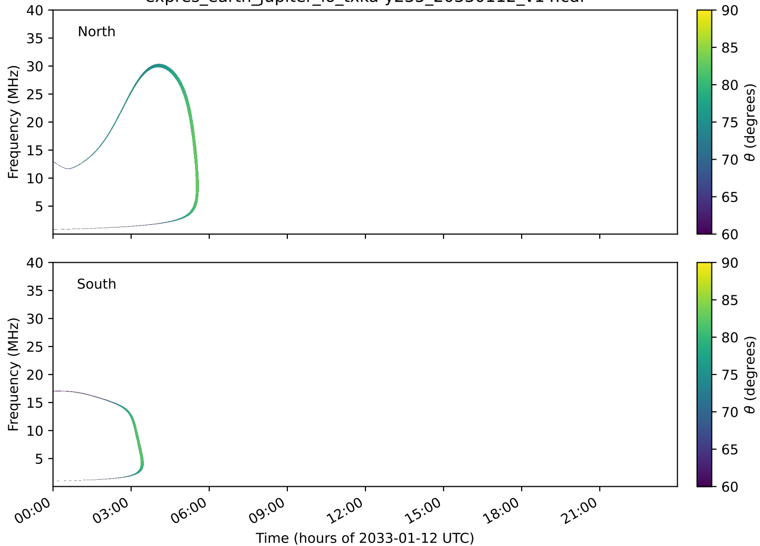
expres_earth_jupiter_io_txka-y235_20330112_v14.cdf
