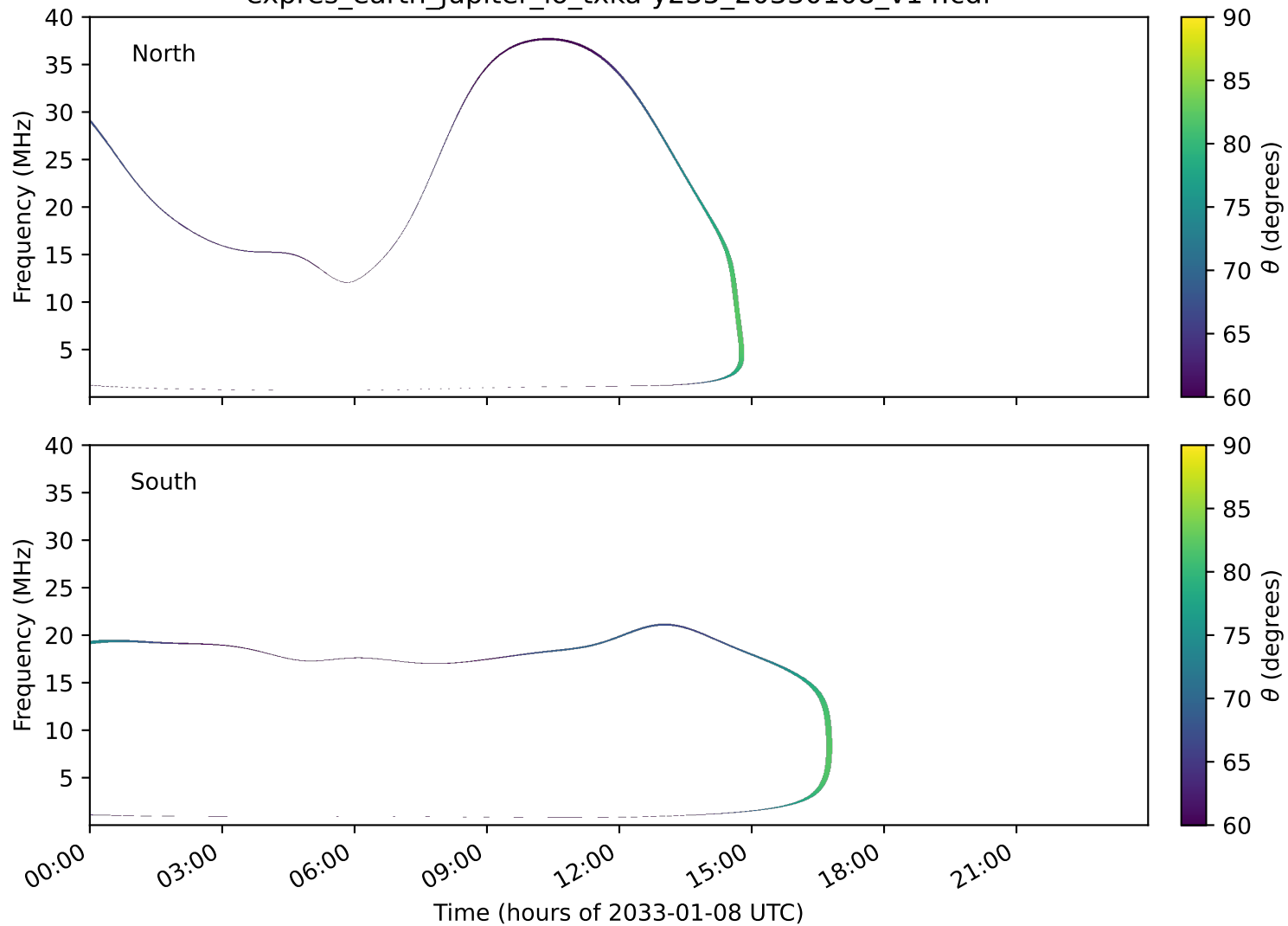
expres_earth_jupiter_io_txka-y235_20330108_v14.cdf
