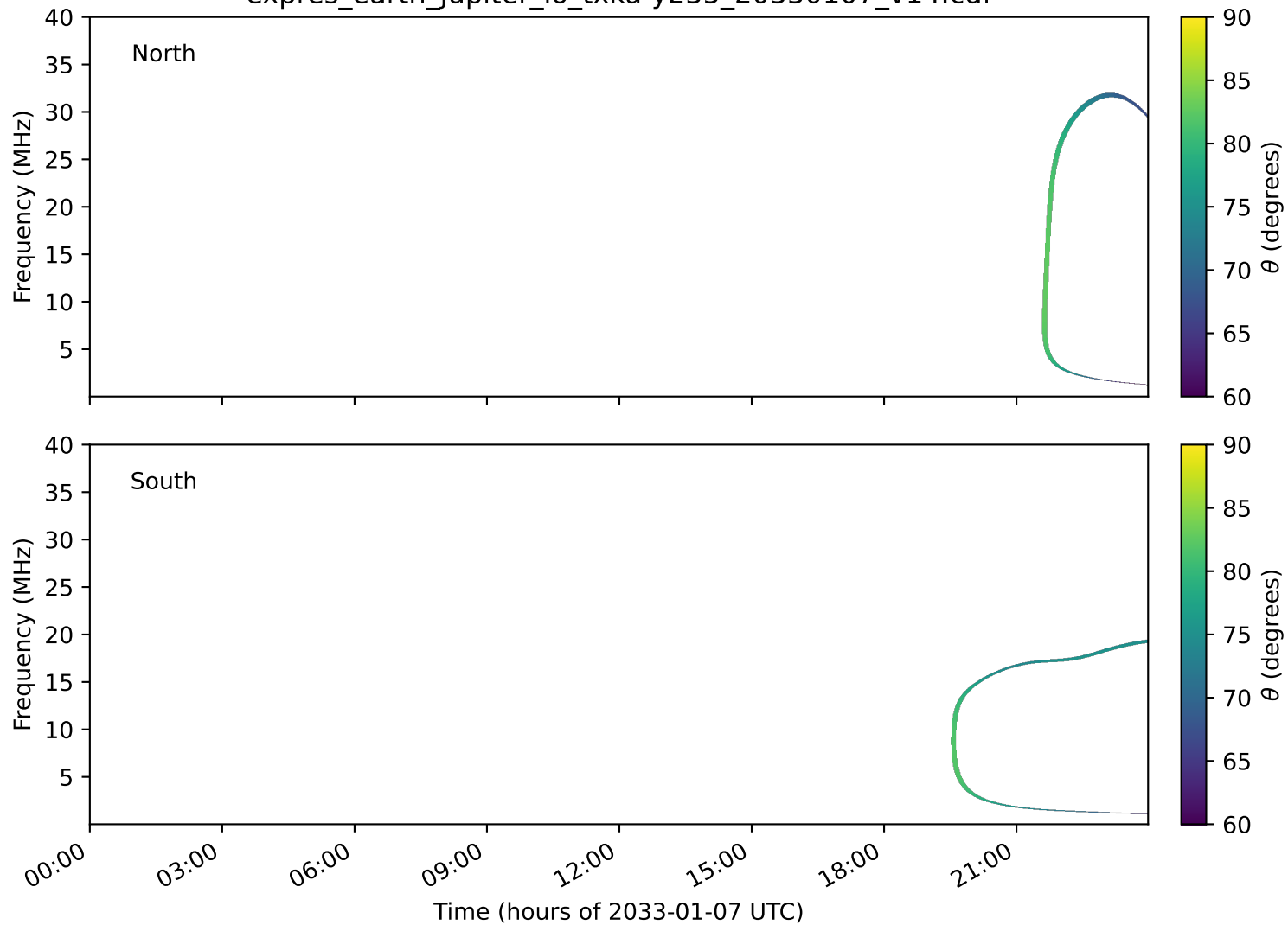
expres_earth_jupiter_io_txka-y235_20330107_v14.cdf
