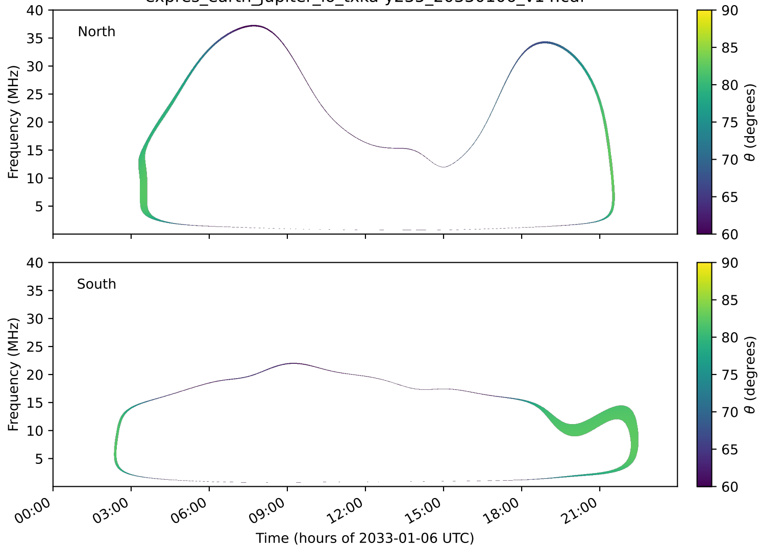
expres_earth_jupiter_io_txka-y235_20330106_v14.cdf
