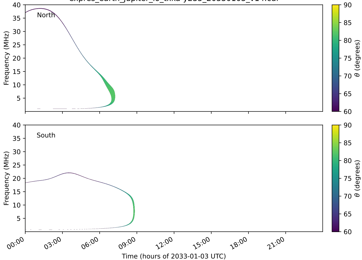
expres_earth_jupiter_io_txka-y235_20330103_v14.cdf
