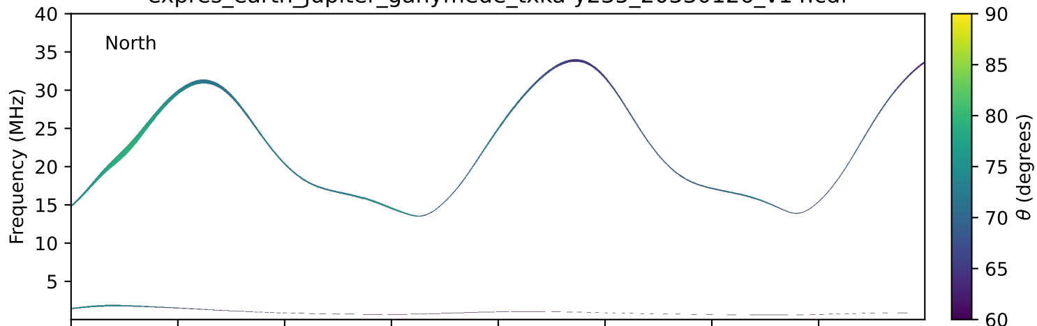
expres_earth_jupiter_ganymede_txka-y235_20330126_v14.cdf
