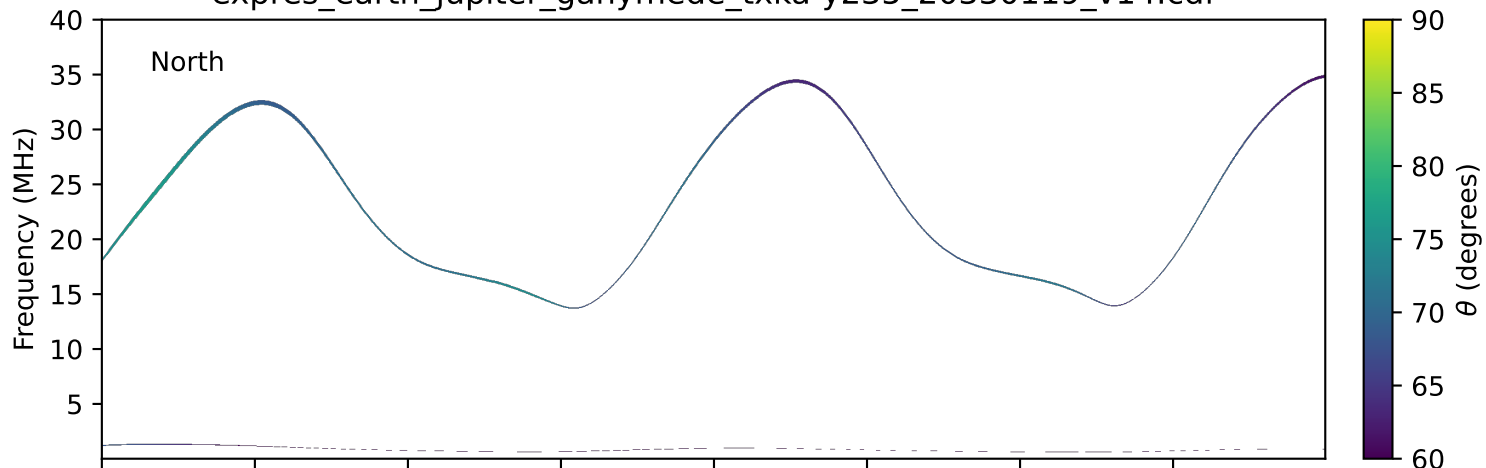
expres_earth_jupiter_ganymede_txka-y235_20330119_v14.cdf
