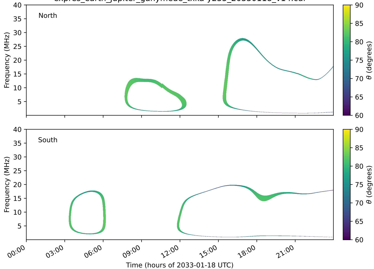
expres_earth_jupiter_ganymede_txka-y235_20330118_v14.cdf
