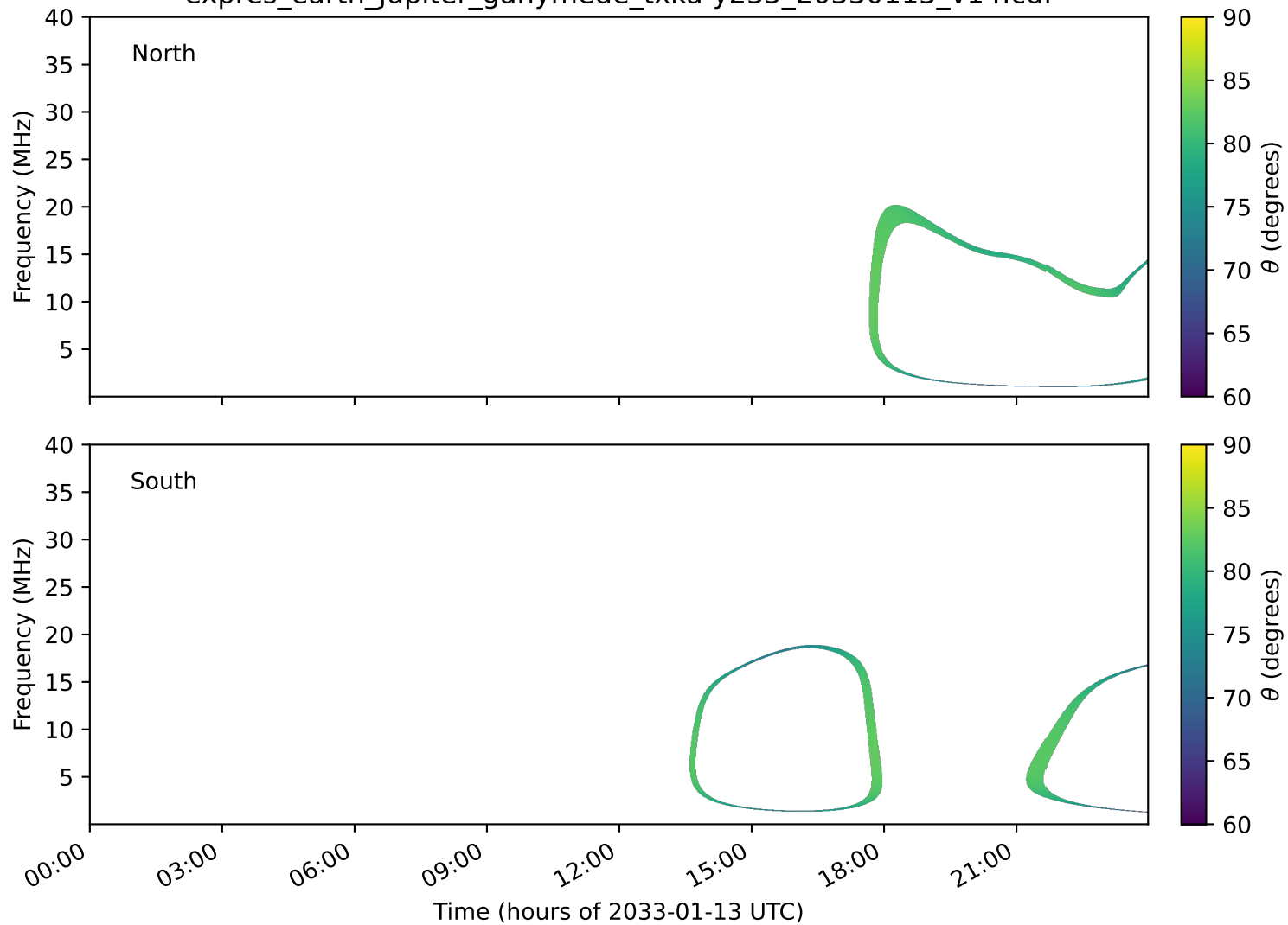
expres_earth_jupiter_ganymede_txka-y235_20330113_v14.cdf
