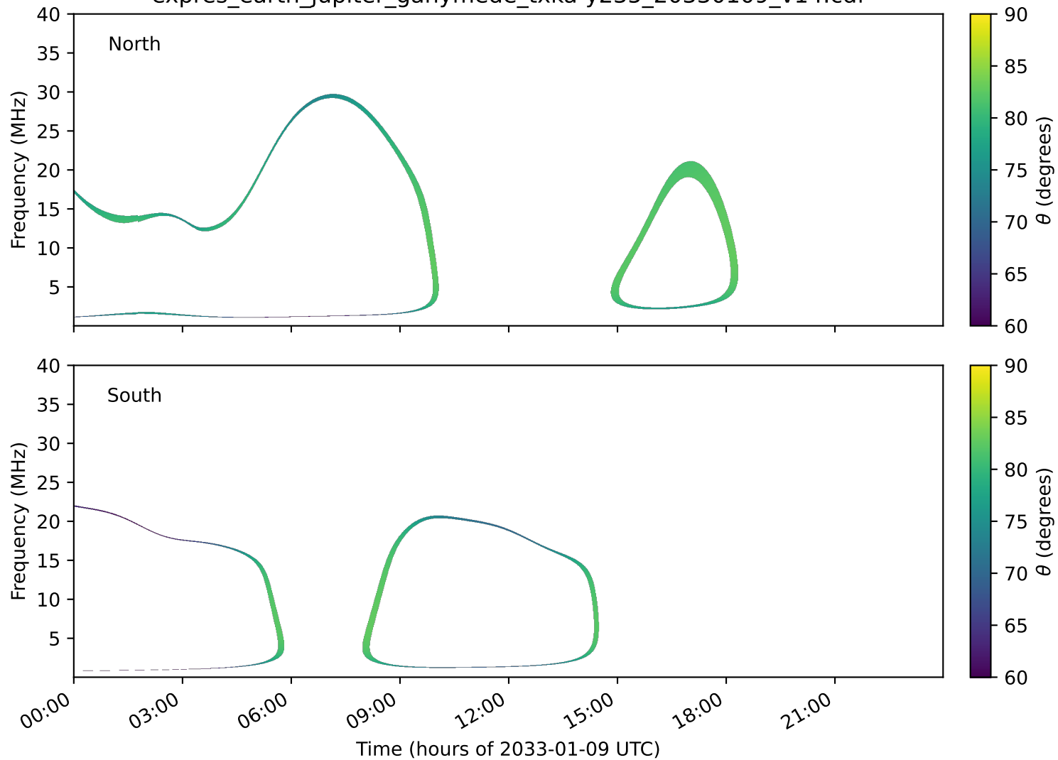
expres_earth_jupiter_ganymede_txka-y235_20330109_v14.cdf
