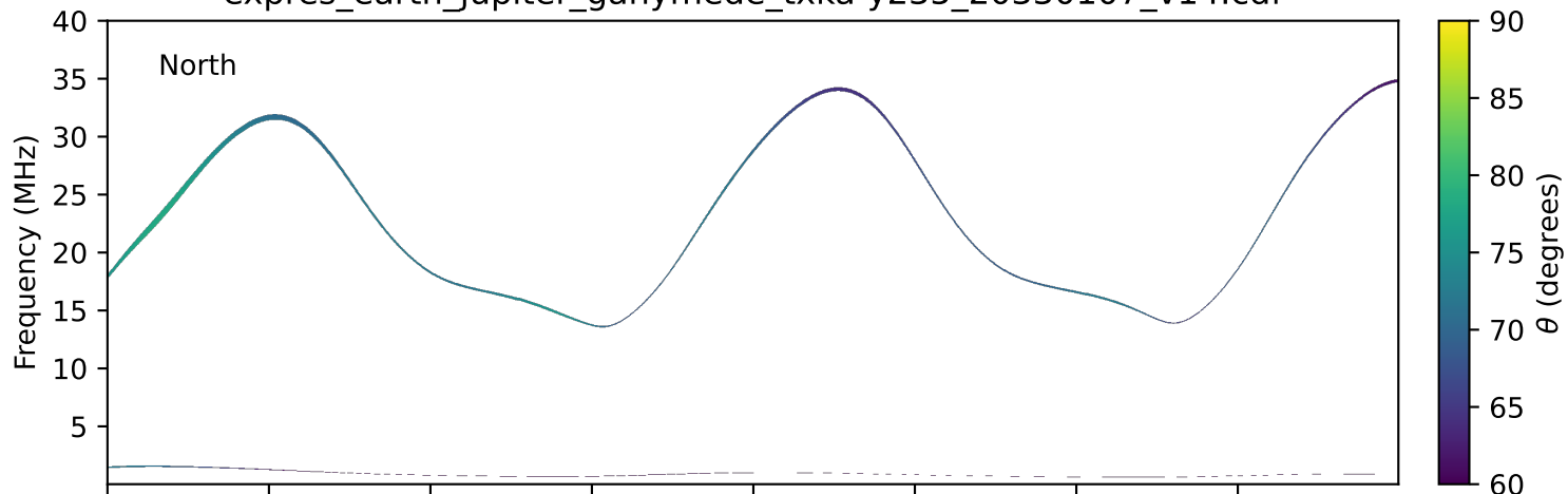
expres_earth_jupiter_ganymede_txka-y235_20330107_v14.cdf
